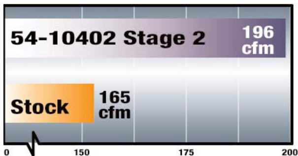
Airflow Comparison (CFM) @ 1.5" H2O
